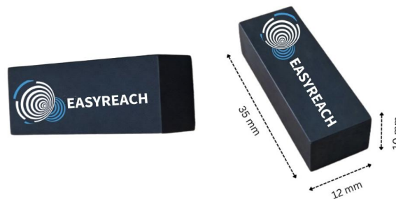
Figure 1 ER-Slick-Mini-Beacon
